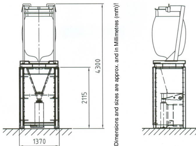
Fig. Dimension PFD 1 WS
